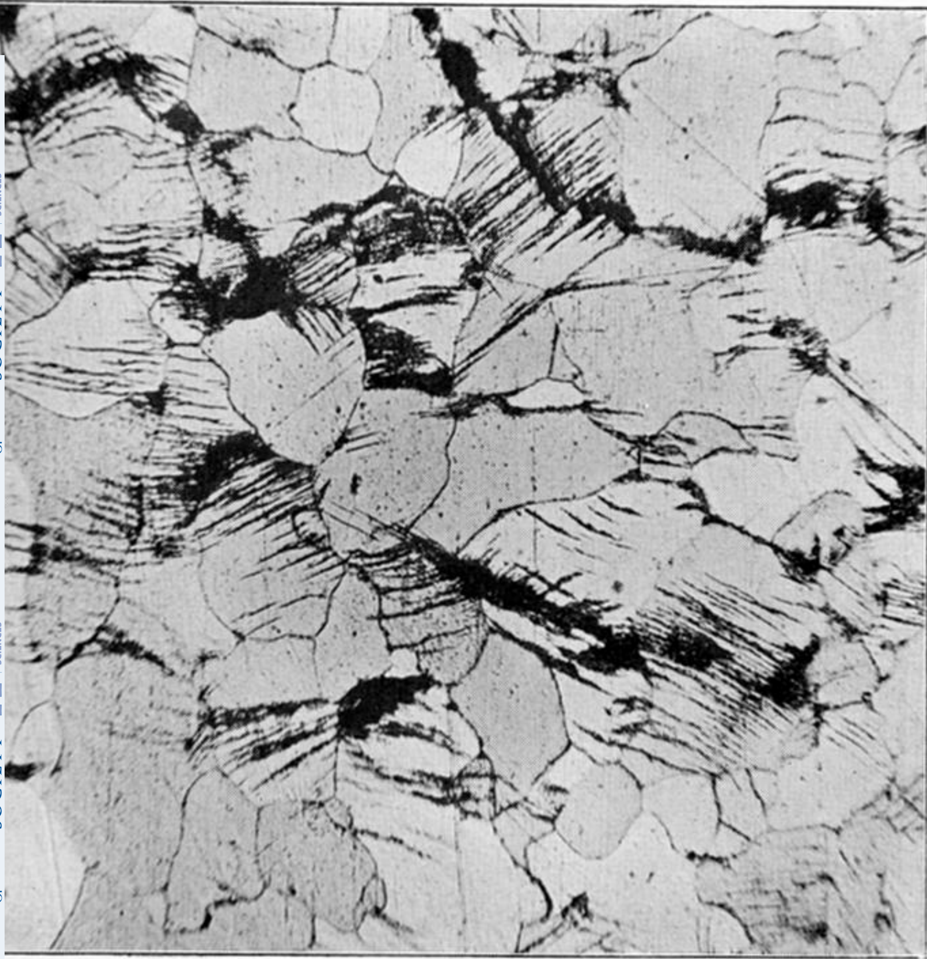
Fig. 5. Same after 60,000 reversals. \times 150 .
