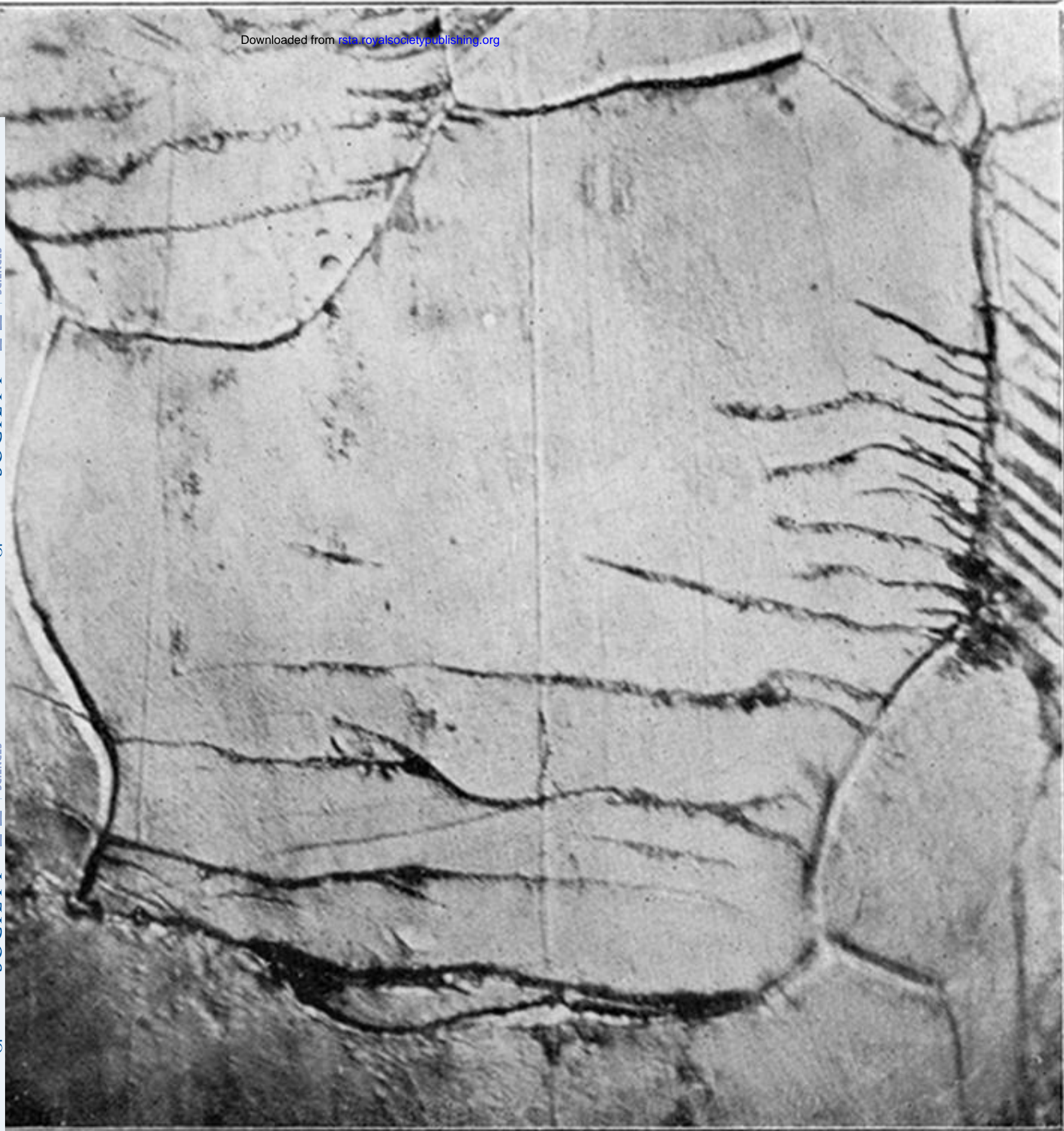
Fig. 12. Same after 40,000 reversals. \times 1000 .
