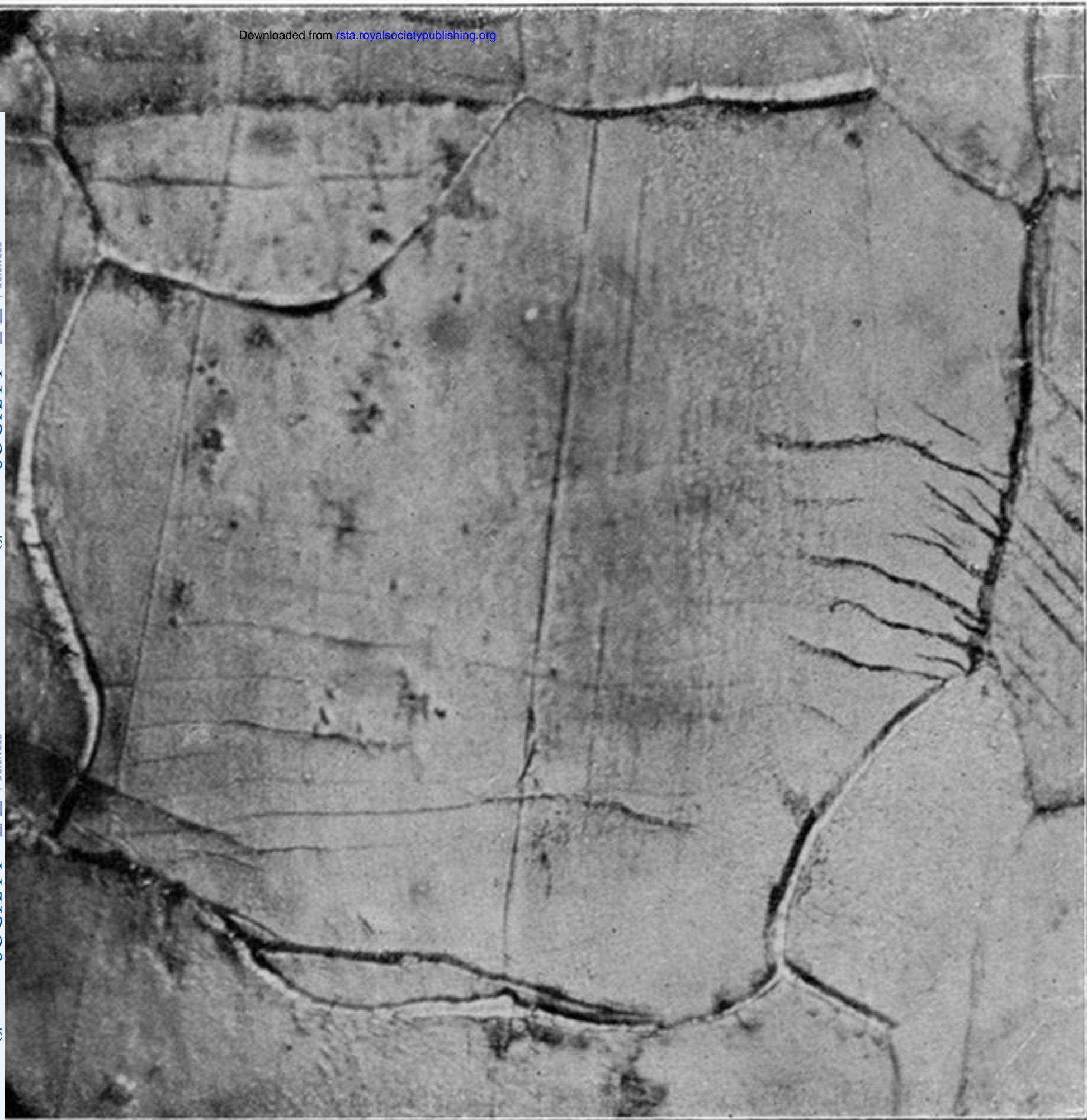
Fig. 11. Same after 10,000 reversals. \times 1000 .
